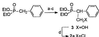
Scheme 2. (a) n -BuLi, THF, -78^{\circ}\text{C} , 15 min; (b) (\text{HCHO})_n , -78^{\circ}\text{C} to rt; (c) \text{H}^+/\text{H}_2\text{O} ; (d) \text{PPh}_3 , \text{CCl}_4 , reflux, 1 h.
